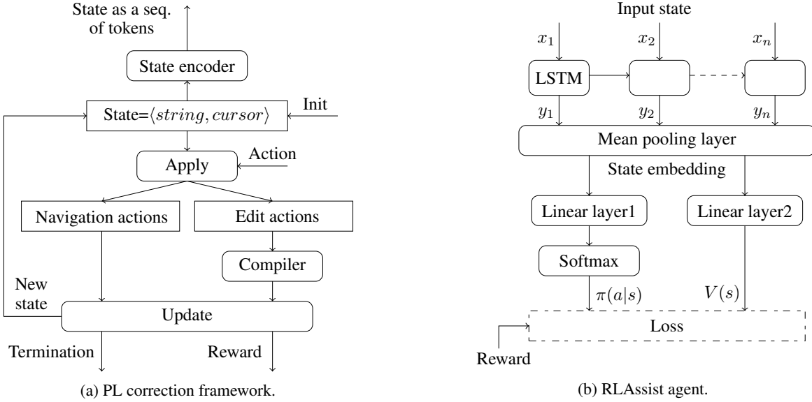
Figure 2: Design of RLAssist.
